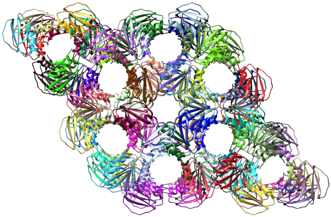
図4.3 Chymotrypsin inhibitor 2の結晶中の並び
